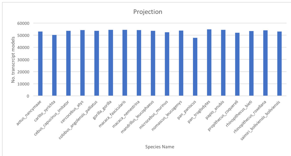
Fig 3: Counts of transcript models build by the projection pipeline for each species
