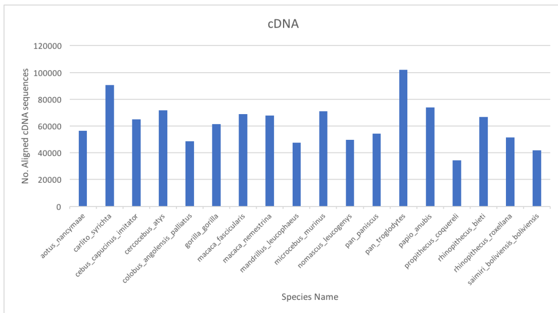
Fig. 2: Counts of cDNA genes in each species
