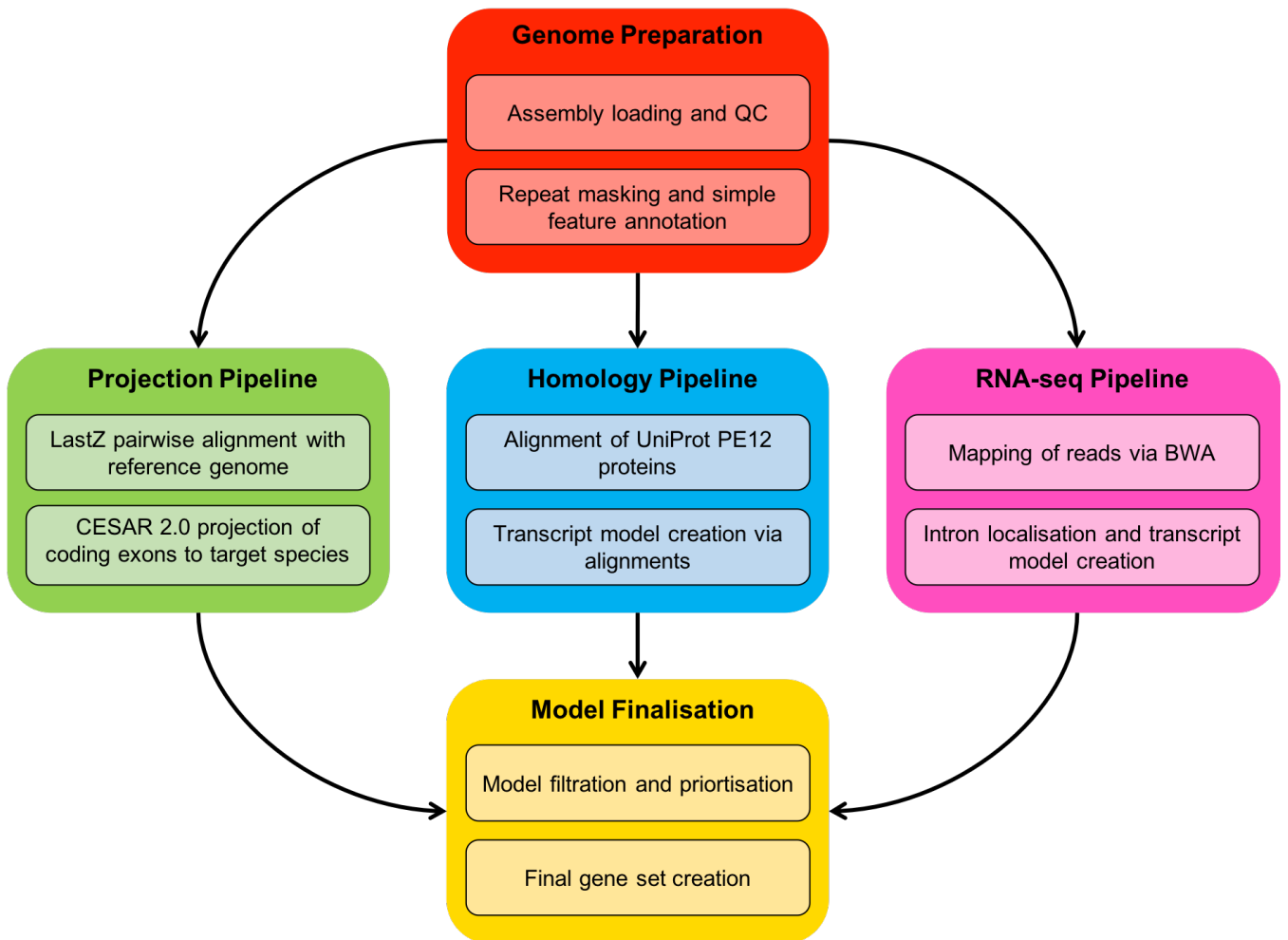
Figure 1: Flowchart of standard protein-coding annotation pipeline. Small ncRNAs, Ig genes, TR genes, and pseudogenes are computed using separate pipelines.
