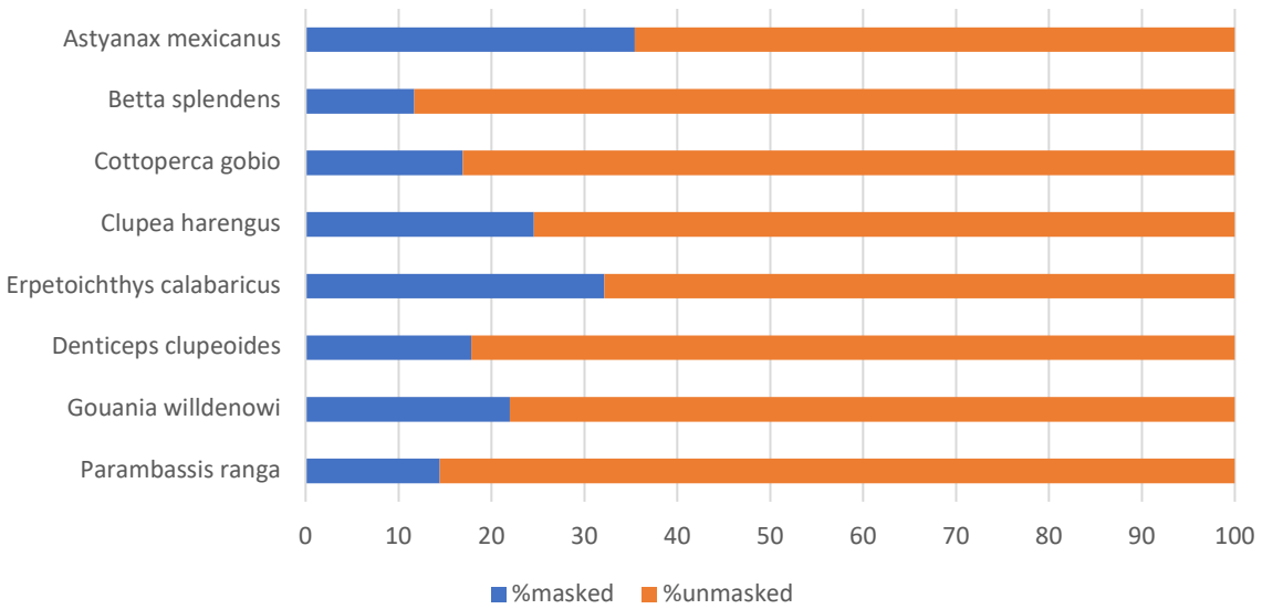
Figure 4: Number of bases repeat masked (blue) and unmasked (orange) per species using the "rebase_teleostei" repeat library.
