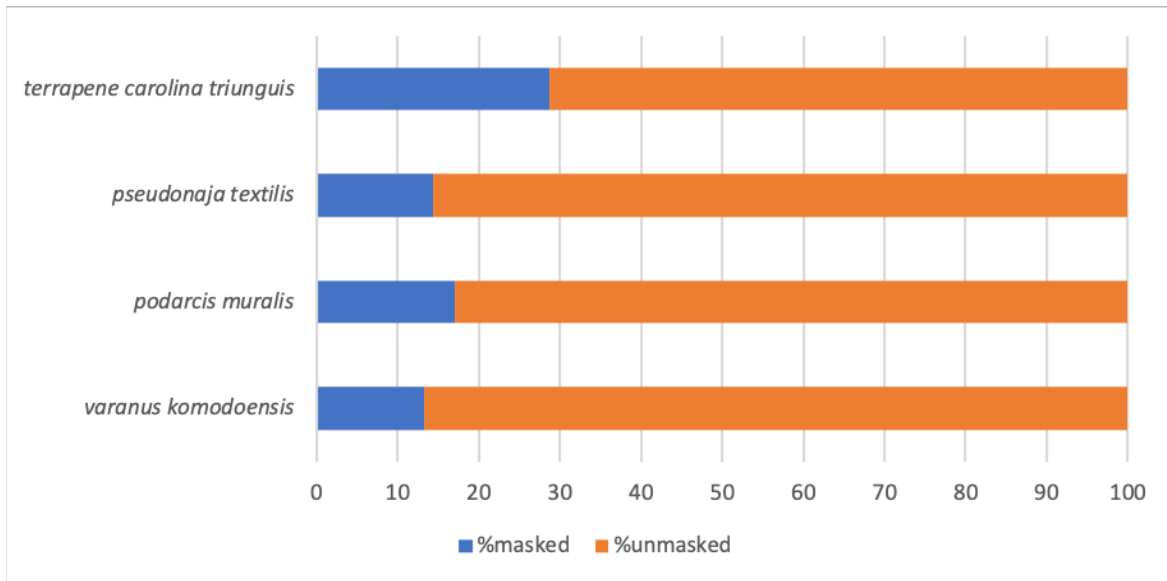
Figure 4: Number of bases repeat masked (blue) and unmasked (orange) per species using the "rebase_vertebrates" repeat library.
