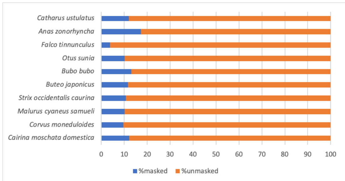
Figure 4: Number of bases repeat masked (blue) and unmasked (orange) per species using the "rebase_birds" repeat library.
