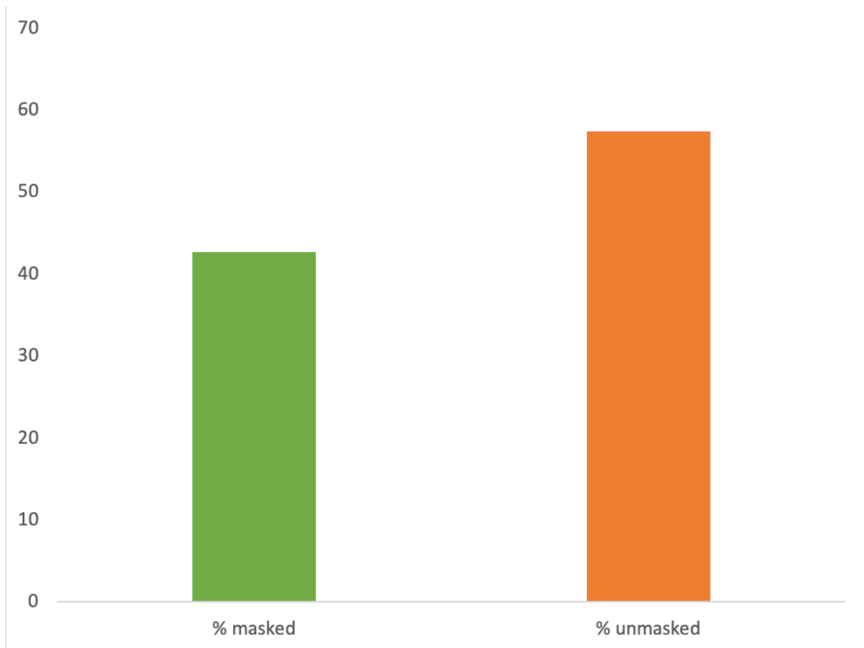
Figure 4: Number of bases repeat masked (green) and unmasked (orange) using the "replibase_mammal" repeat library.
