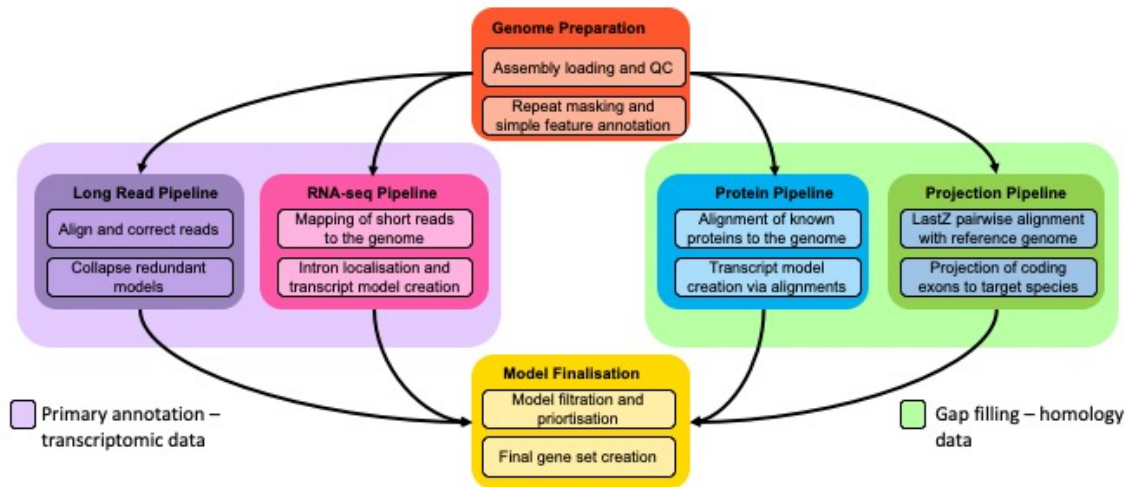
Fig. 1: Flowchart of the protein-coding annotation pipeline. Small ncRNAs, Ig genes, TR genes, and pseudogenes are computed using separate pipelines.
